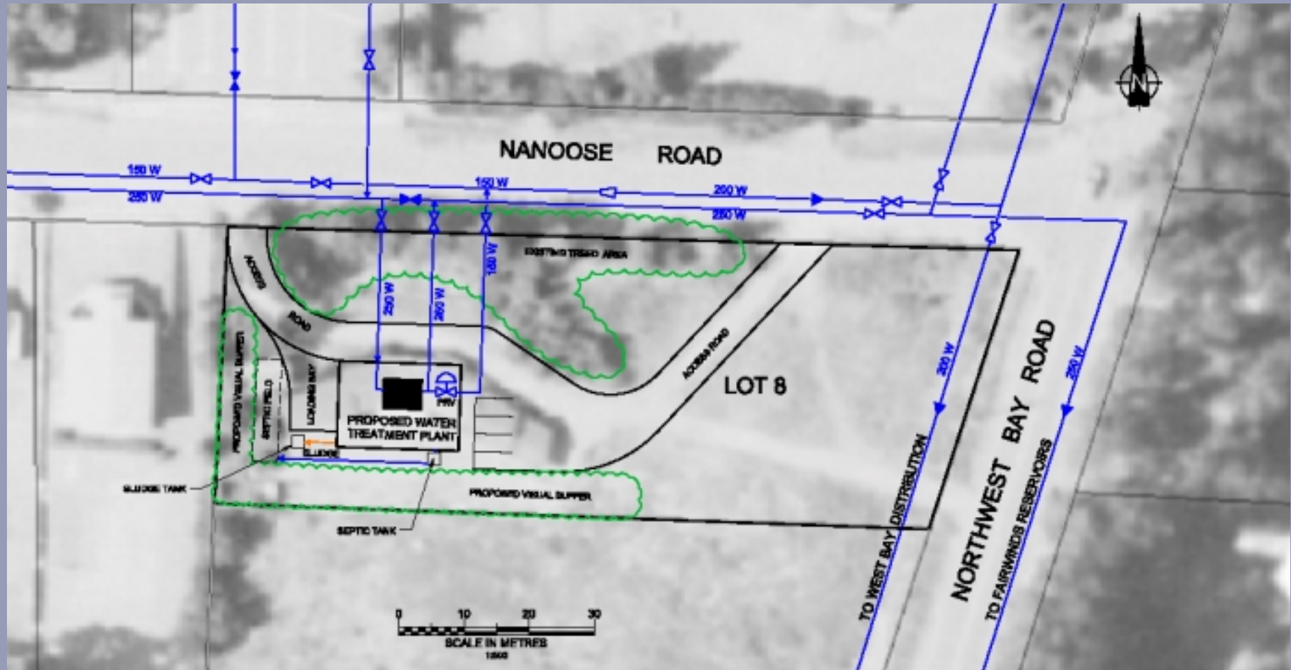
Nanoose Bay Peninsula Water Service Area - Proposed Water Treatment Facility
